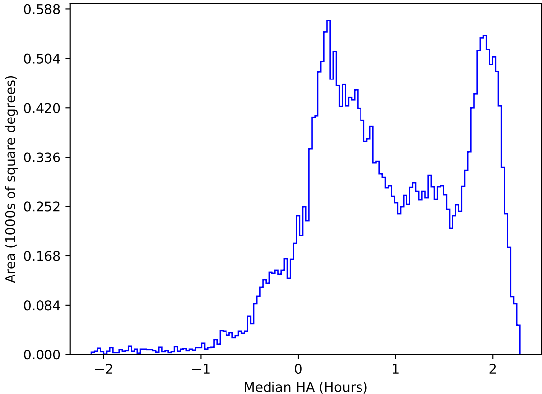
ddf_acor_sf30_lsf40_lsr20_v3.4_10yrs All sky all bands: Median HA
