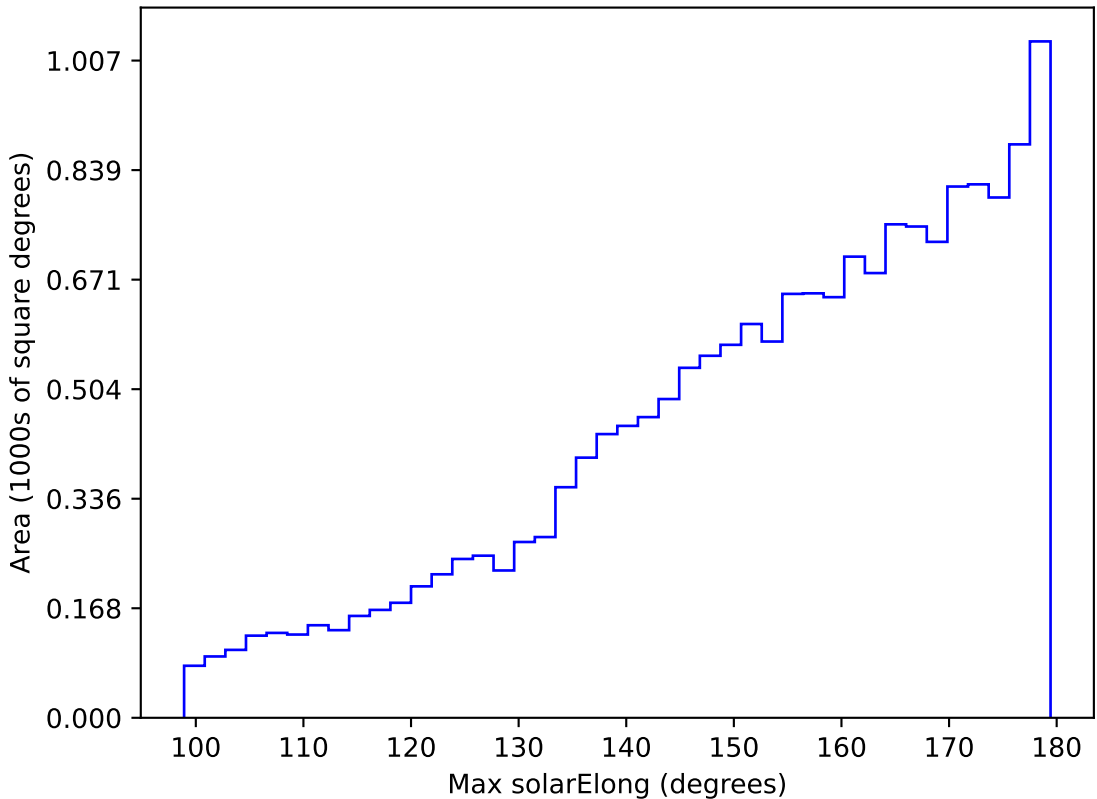
ddf_acor_sf30_lsf40_lsr20_v3.4_10yrs WFD z band: Max solarElong
