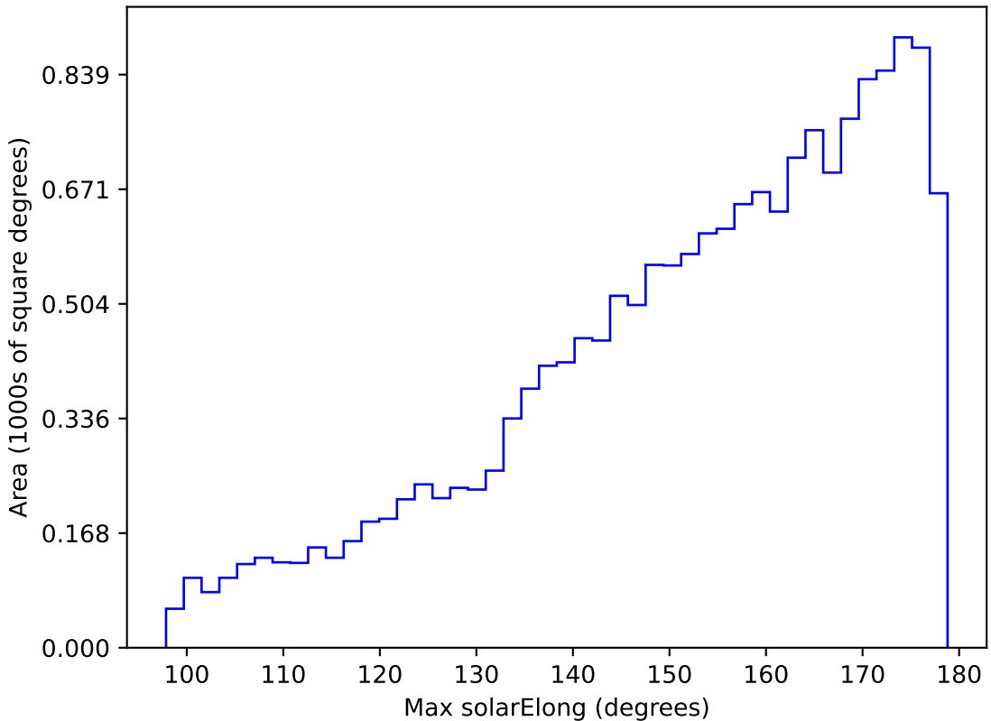
ddf_acor_sf30_lsf40_lsr20_v3.4_10yrs WFD u band: Max solarElong
