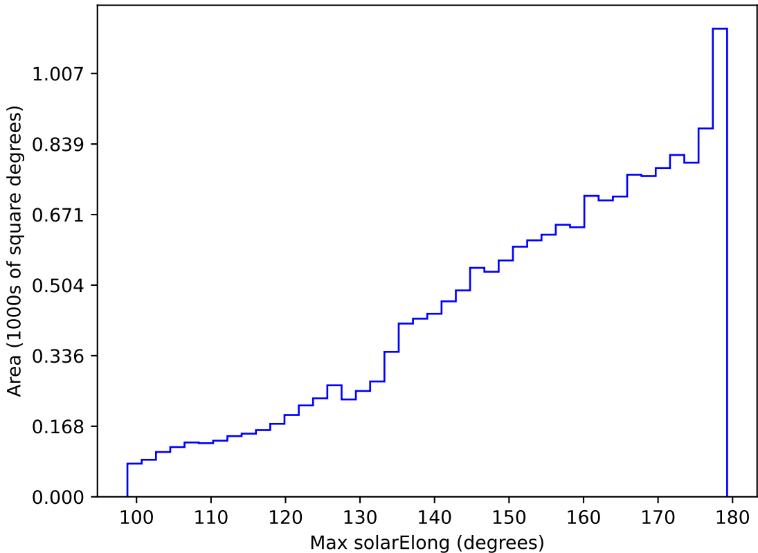
ddf_acor_sf30_lsf40_lsr20_v3.4_10yrs WFD r band: Max solarElong
