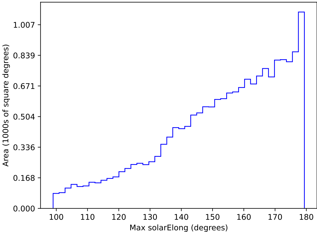
ddf_acor_sf30_lsf40_lsr20_v3.4_10yrs WFD i band: Max solarElong
