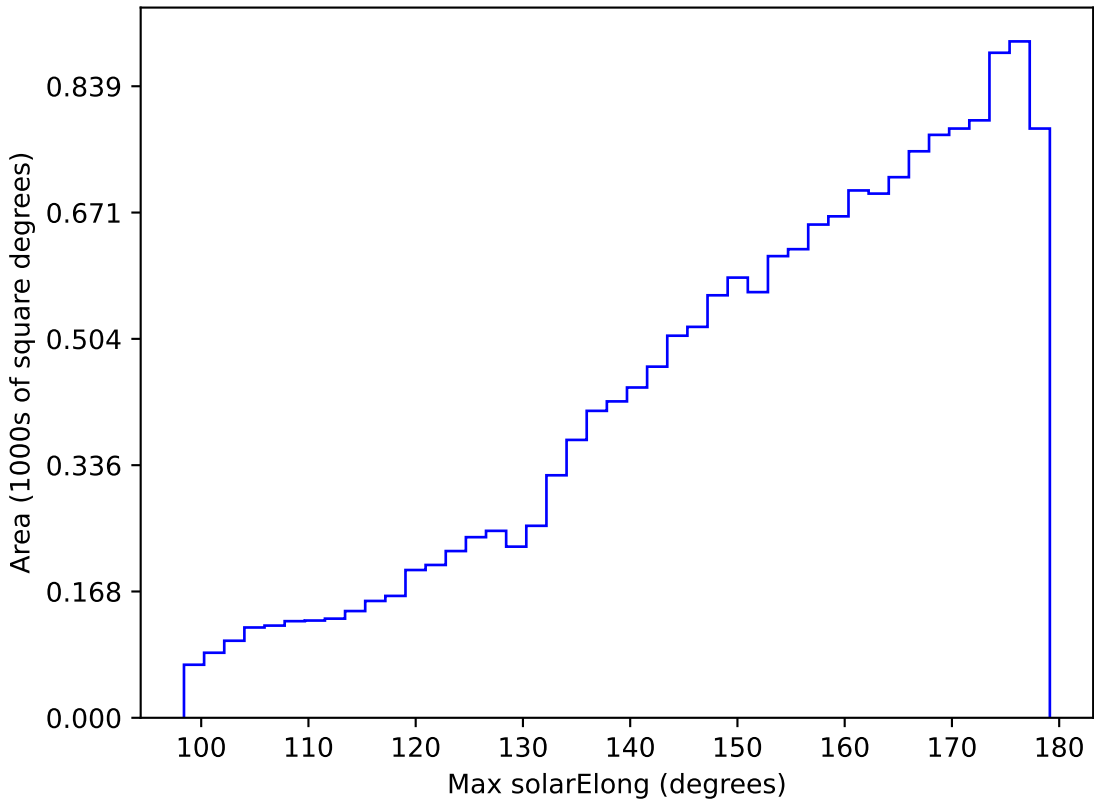
ddf_acor_sf30_lsf40_lsr20_v3.4_10yrs WFD g band: Max solarElong
