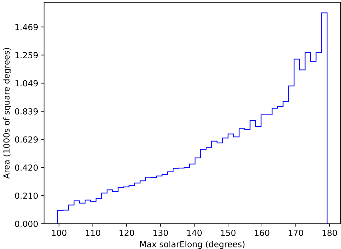
ddf_acor_sf30_lsf40_lsr20_v3.4_10yrs All sky r band: Max solarElong
