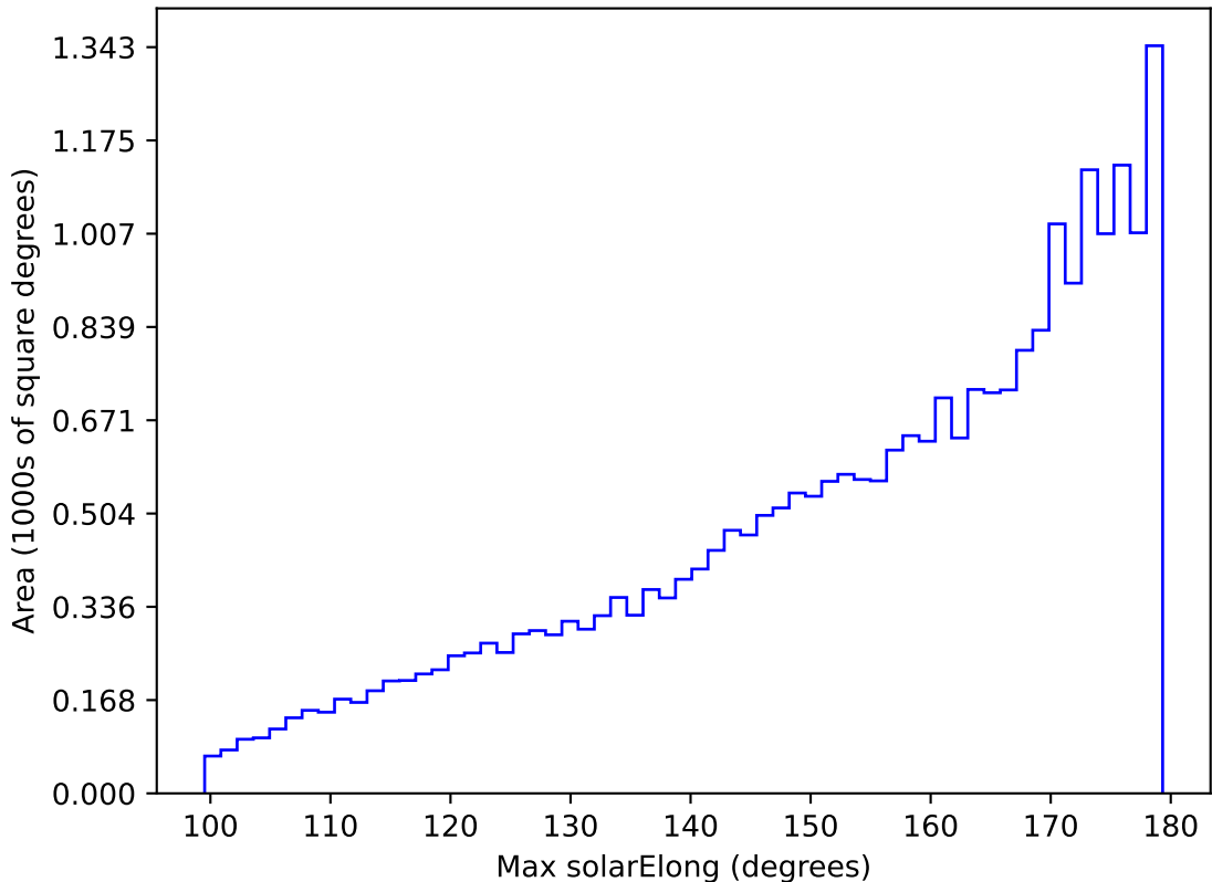
ddf_acor_sf30_lsf40_lsr20_v3.4_10yrs All sky i band: Max solarElong
