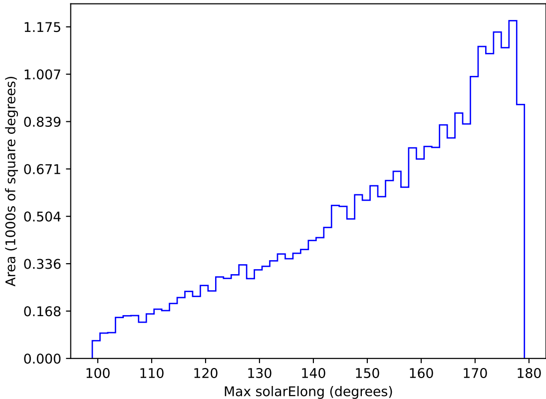
ddf_acor_sf30_lsf40_lsr20_v3.4_10yrs All sky g band: Max solarElong
