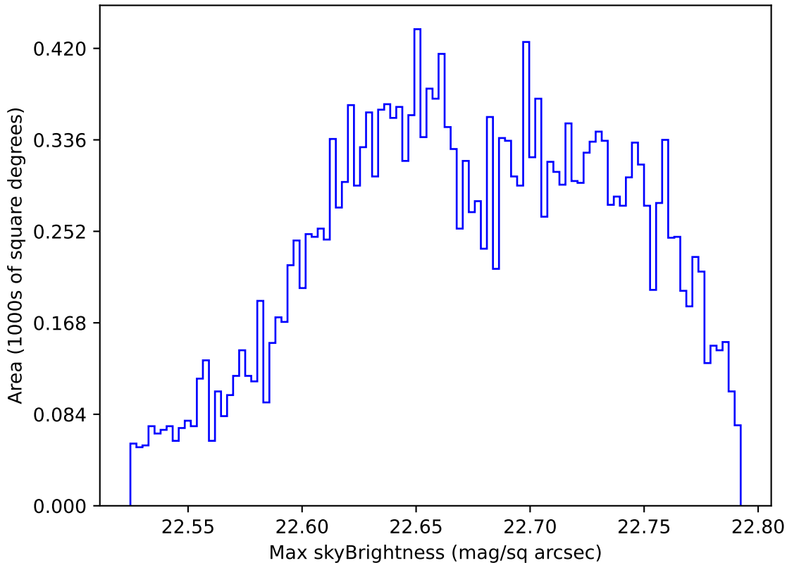
ddf_acor_sf30_lsf40_lsr20_v3.4_10yrs Yr 1 u band: Max skyBrightness
