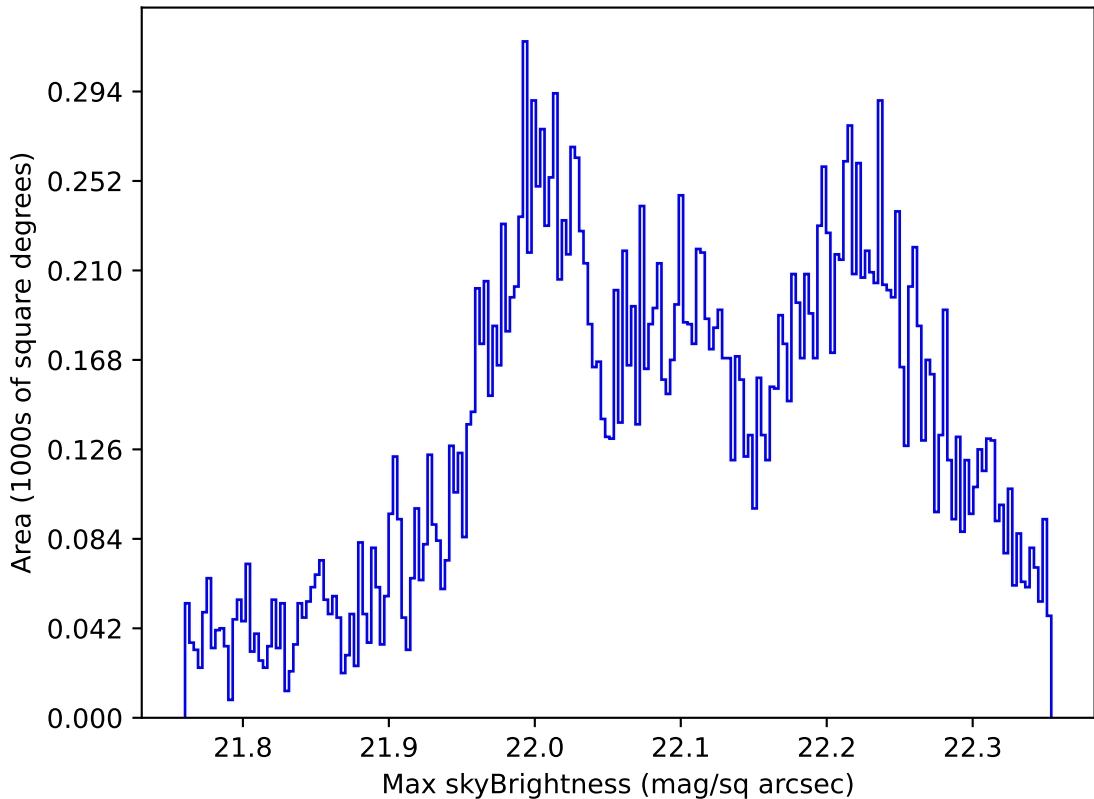
ddf_acor_sf30_lsf40_lsr20_v3.4_10yrs Yr 1 g band: Max skyBrightness
