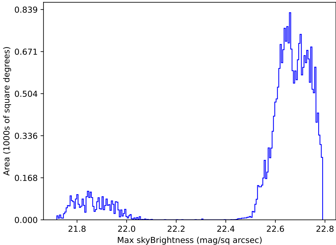
ddf_acor_sf30_lsf40_lsr20_v3.4_10yrs Yr 1 all bands: Max skyBrightness
