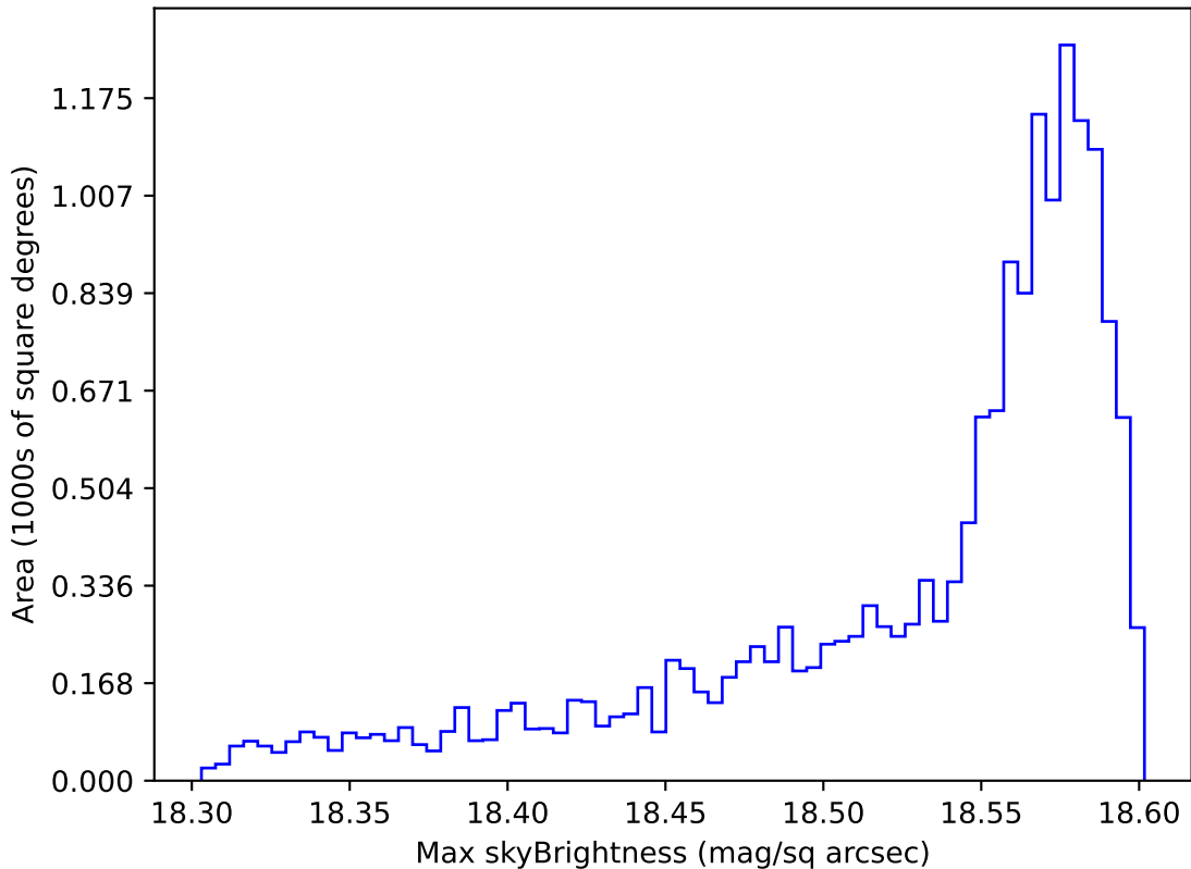
ddf_acor_sf30_lsf40_lsr20_v3.4_10yrs WFD y band: Max skyBrightness
