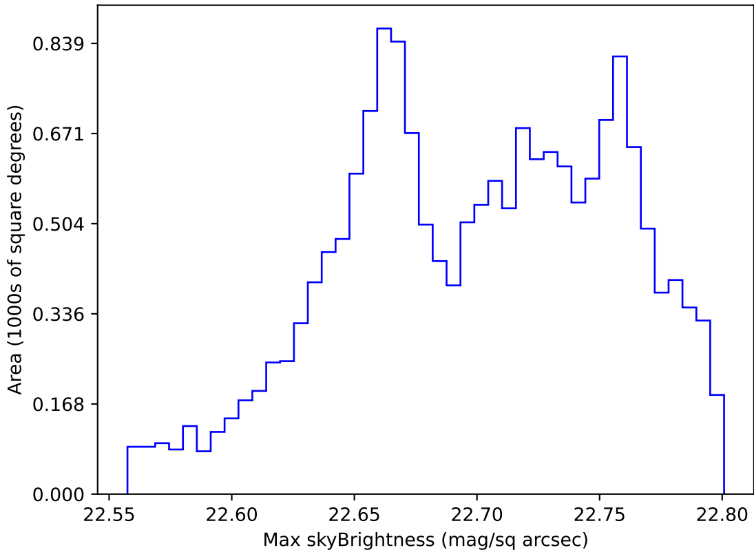
ddf_acor_sf30_lsf40_lsr20_v3.4_10yrs WFD u band: Max skyBrightness
