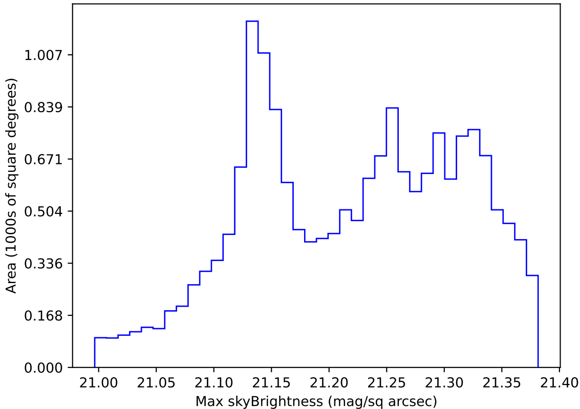
ddf_acor_sf30_lsf40_lsr20_v3.4_10yrs WFD r band: Max skyBrightness
