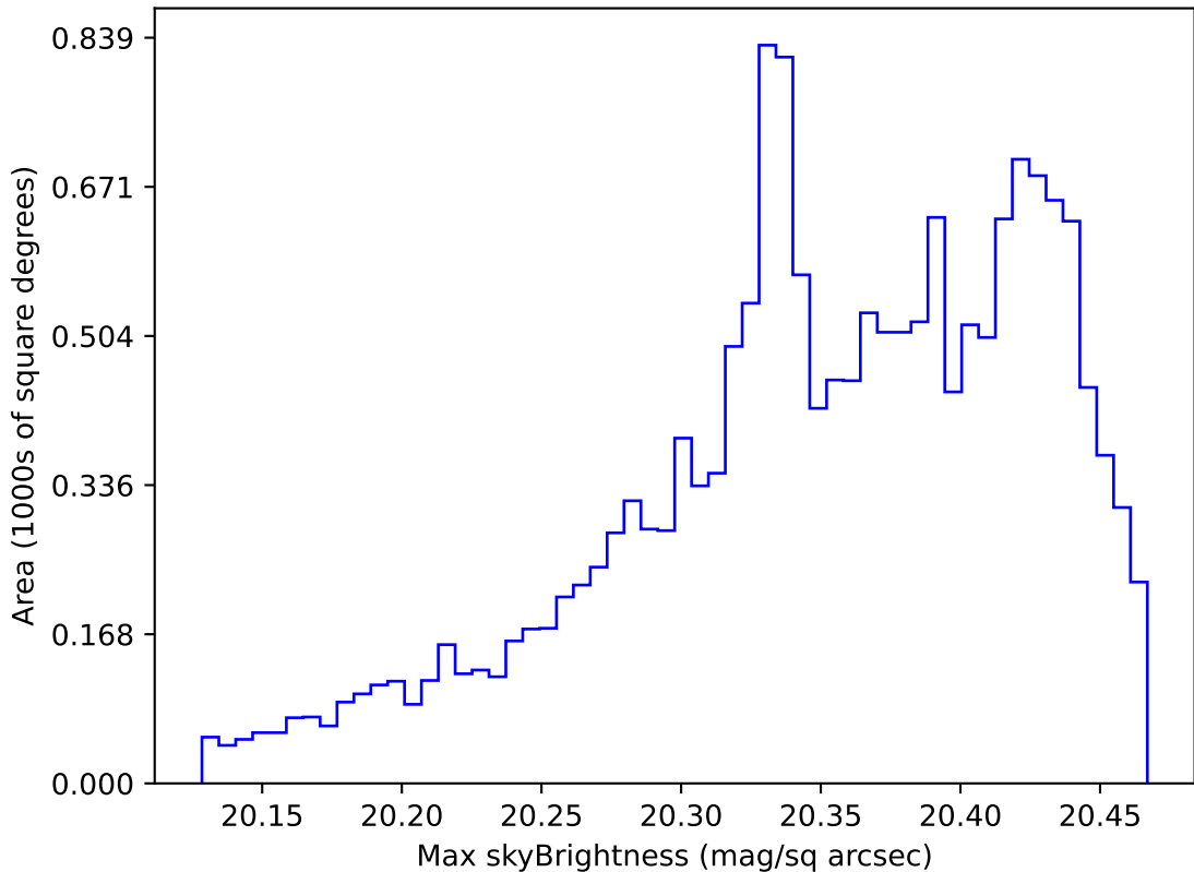
ddf_acor_sf30_lsf40_lsr20_v3.4_10yrs WFD i band: Max skyBrightness
