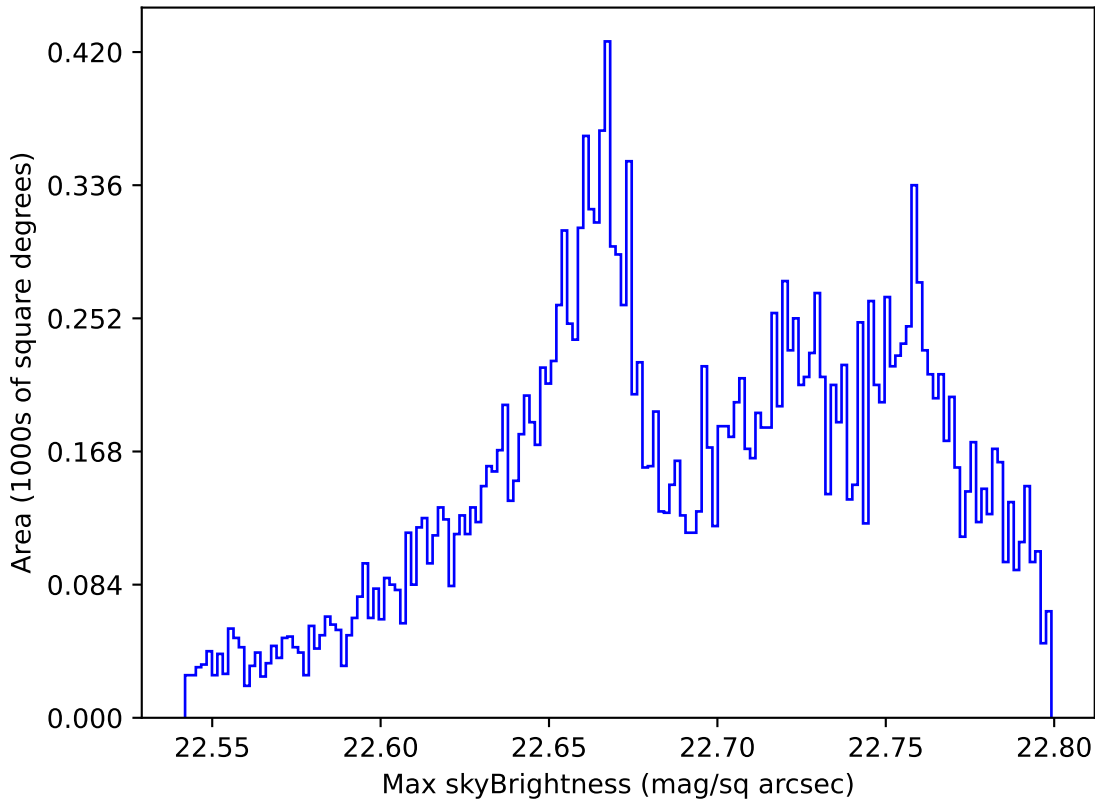
ddf_acor_sf30_lsf40_lsr20_v3.4_10yrs All sky u band: Max skyBrightness
