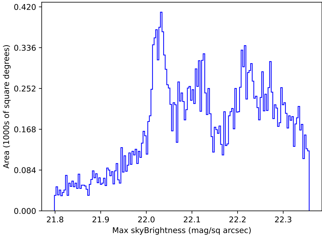
ddf_acor_sf30_lsf40_lsr20_v3.4_10yrs All sky g band: Max skyBrightness
