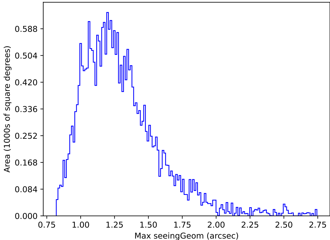
ddf_acor_sf30_lsf40_lsr20_v3.4_10yrs Yr 1 z band: Max seeingGeom
