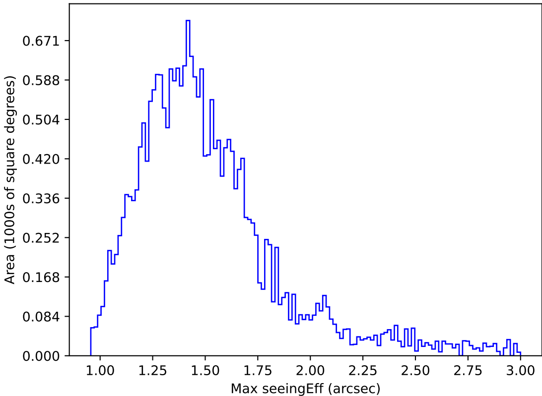
ddf_acor_sf30_lsf40_lsr20_v3.4_10yrs Yr 1 y band: Max seeingEff
