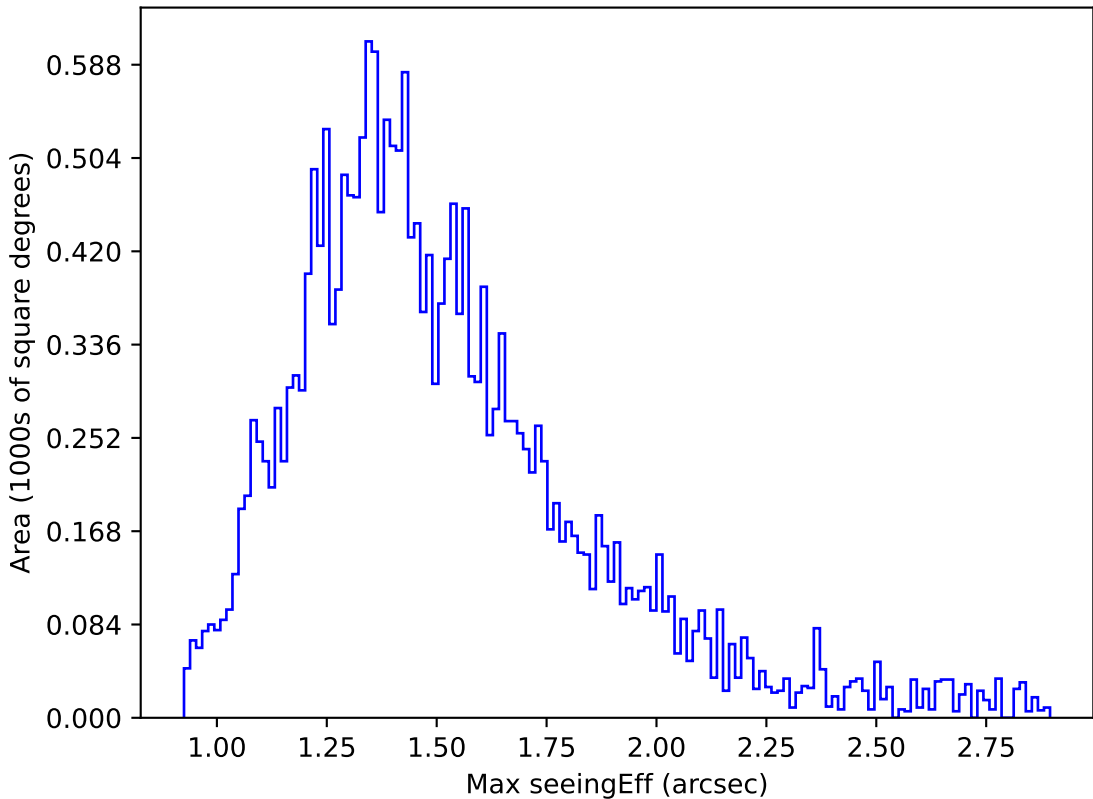
ddf_acor_sf30_lsf40_lsr20_v3.4_10yrs Yr 1 u band: Max seeingEff
