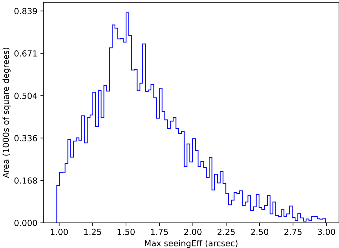
ddf_acor_sf30_lsf40_lsr20_v3.4_10yrs Yr 1 r band: Max seeingEff
