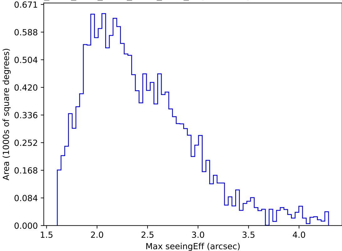
ddf_acor_sf30_lsf40_lsr20_v3.4_10yrs WFD y band: Max seeingEff
