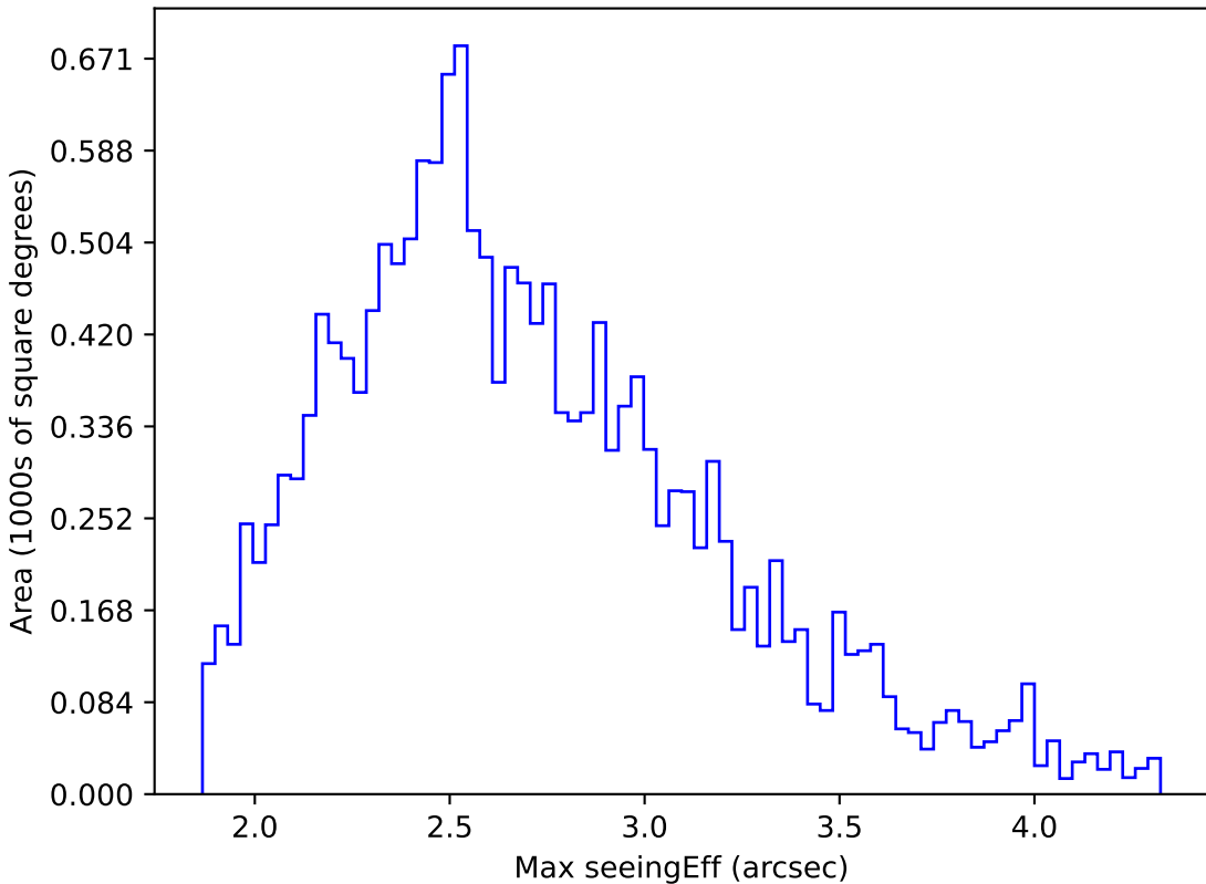
ddf_acor_sf30_lsf40_lsr20_v3.4_10yrs WFD r band: Max seeingEff
