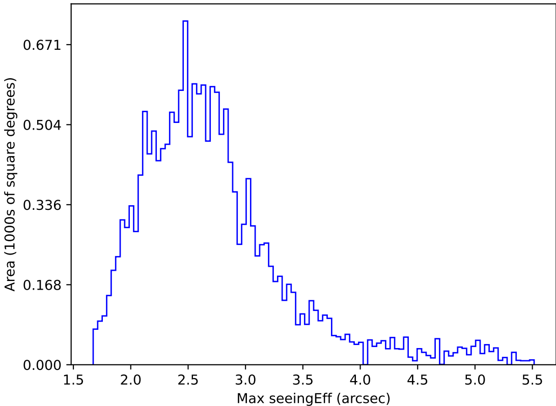
ddf_acor_sf30_lsf40_lsr20_v3.4_10yrs WFD i band: Max seeingEff
