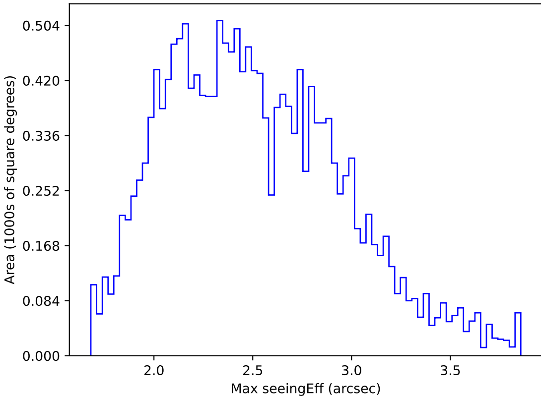
ddf_acor_sf30_lsf40_lsr20_v3.4_10yrs WFD g band: Max seeingEff
