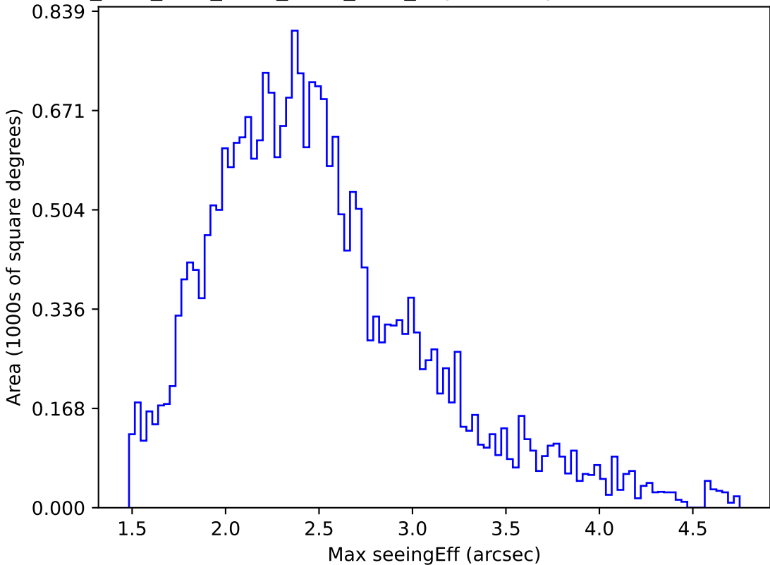
ddf_acor_sf30_lsf40_lsr20_v3.4_10yrs All sky z band: Max seeingEff
