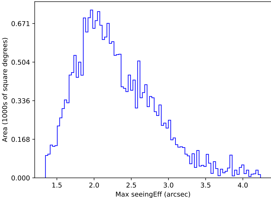
ddf_acor_sf30_ls40_lsr20_v3.4_10yrs All sky y band: Max seeingEff
