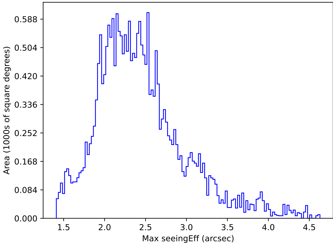
ddf_acor_sf30_ls40_lsr20_v3.4_10yrs All sky u band: Max seeingEff
