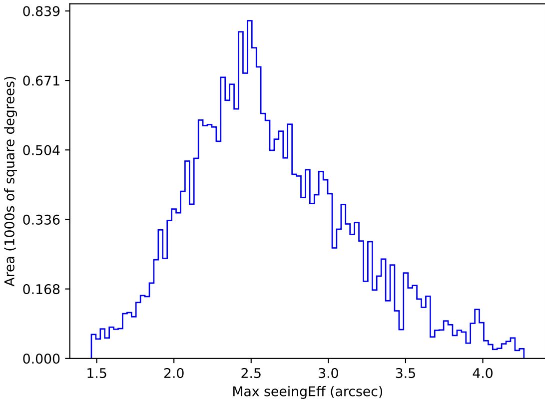
ddf_acor_sf30_lsf40_lsr20_v3.4_10yrs All sky r band: Max seeingEff
