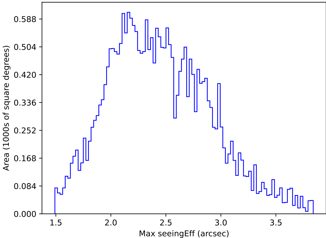
ddf_acor_sf30_ls40_lsr20_v3.4_10yrs All sky g band: Max seeingEff
