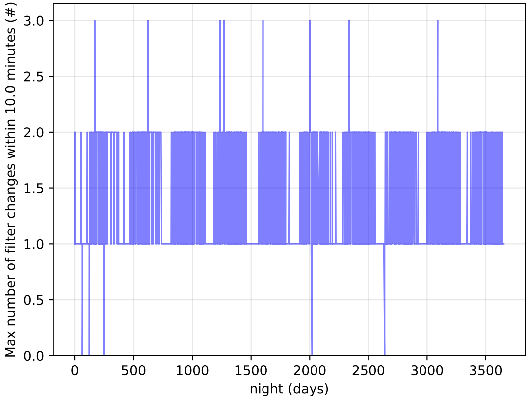
ddf_acor_sf30_Isf40_Isr20_v3.4_10yrs Per Night: Max number of filter changes within 10.0 minutes
