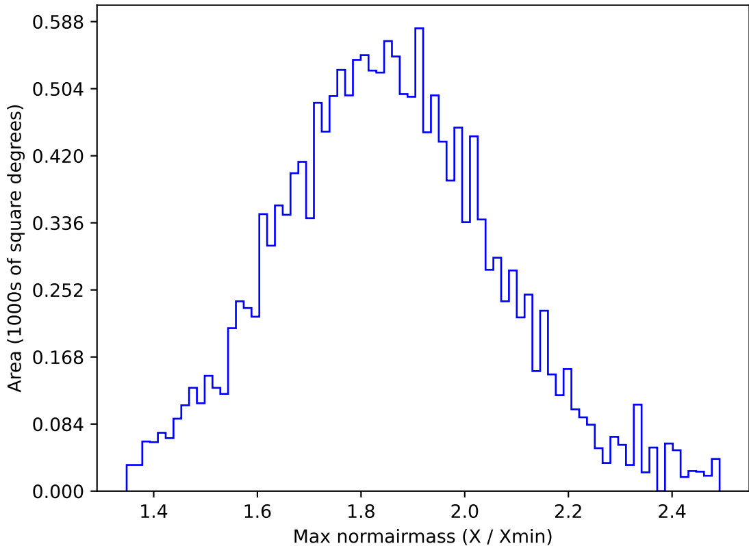
ddf_acor_sf30_lsf40_lsr20_v3.4_10yrs WFD g band: Max normairmass
