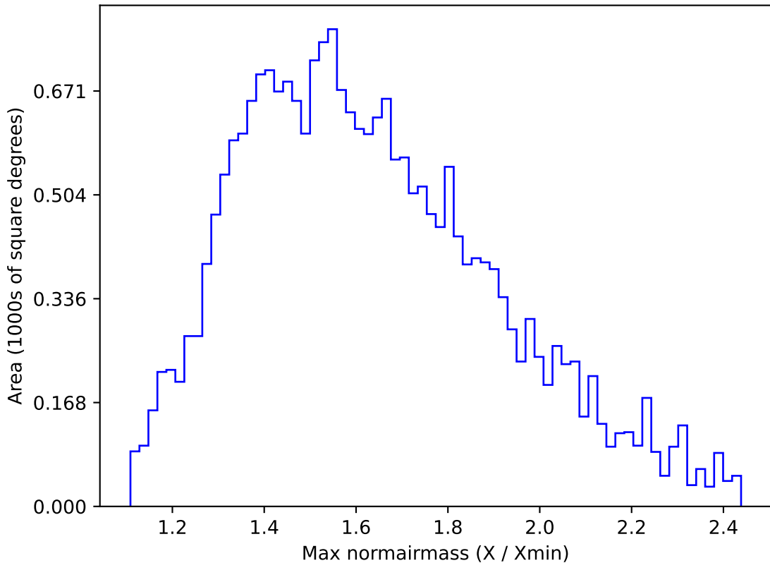
ddf_acor_sf30_lsf40_lsr20_v3.4_10yrs All sky u band: Max normairmass
