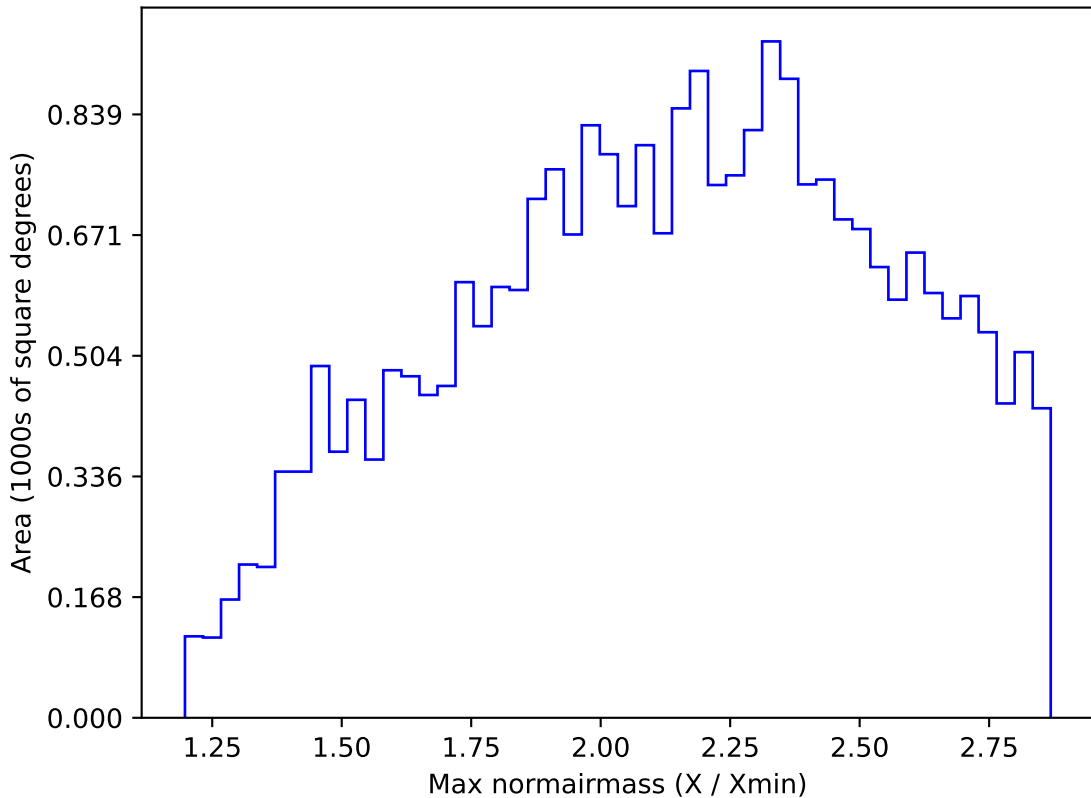
ddf_acor_sf30_lsf40_lsr20_v3.4_10yrs All sky i band: Max normairmass
