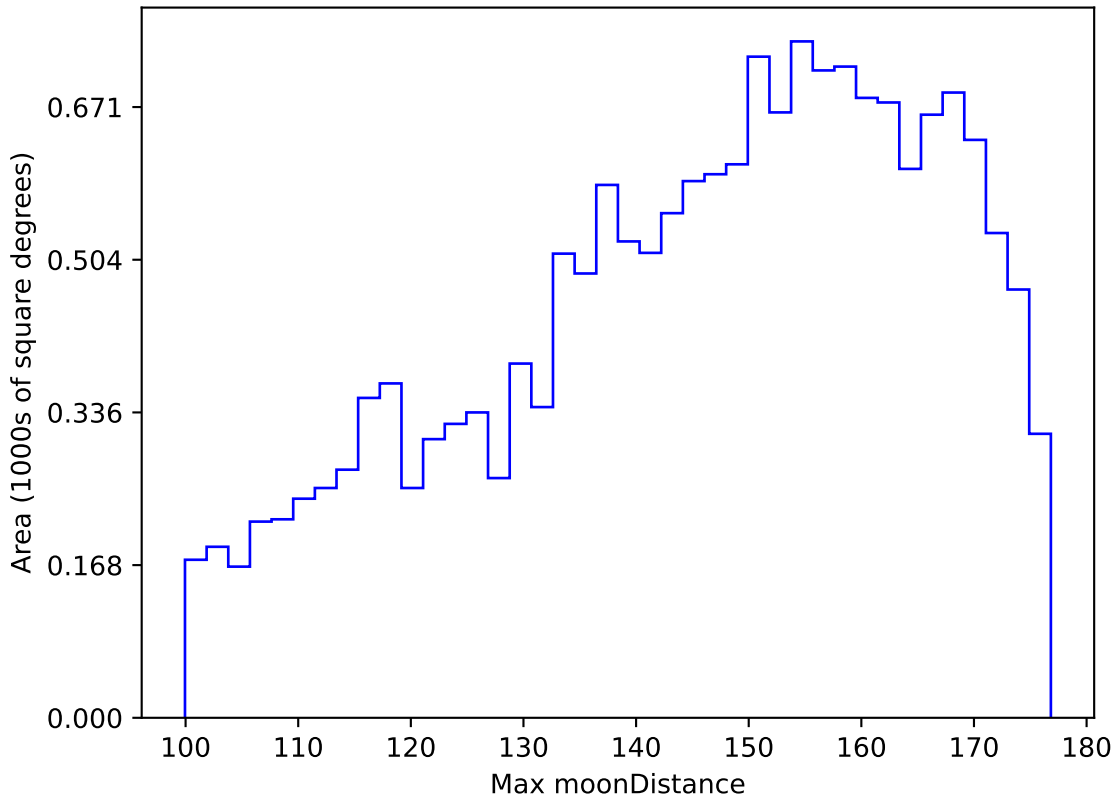
ddf_acor_sf30_lsf40_lsr20_v3.4_10yrs WFD y band: Max moonDistance
