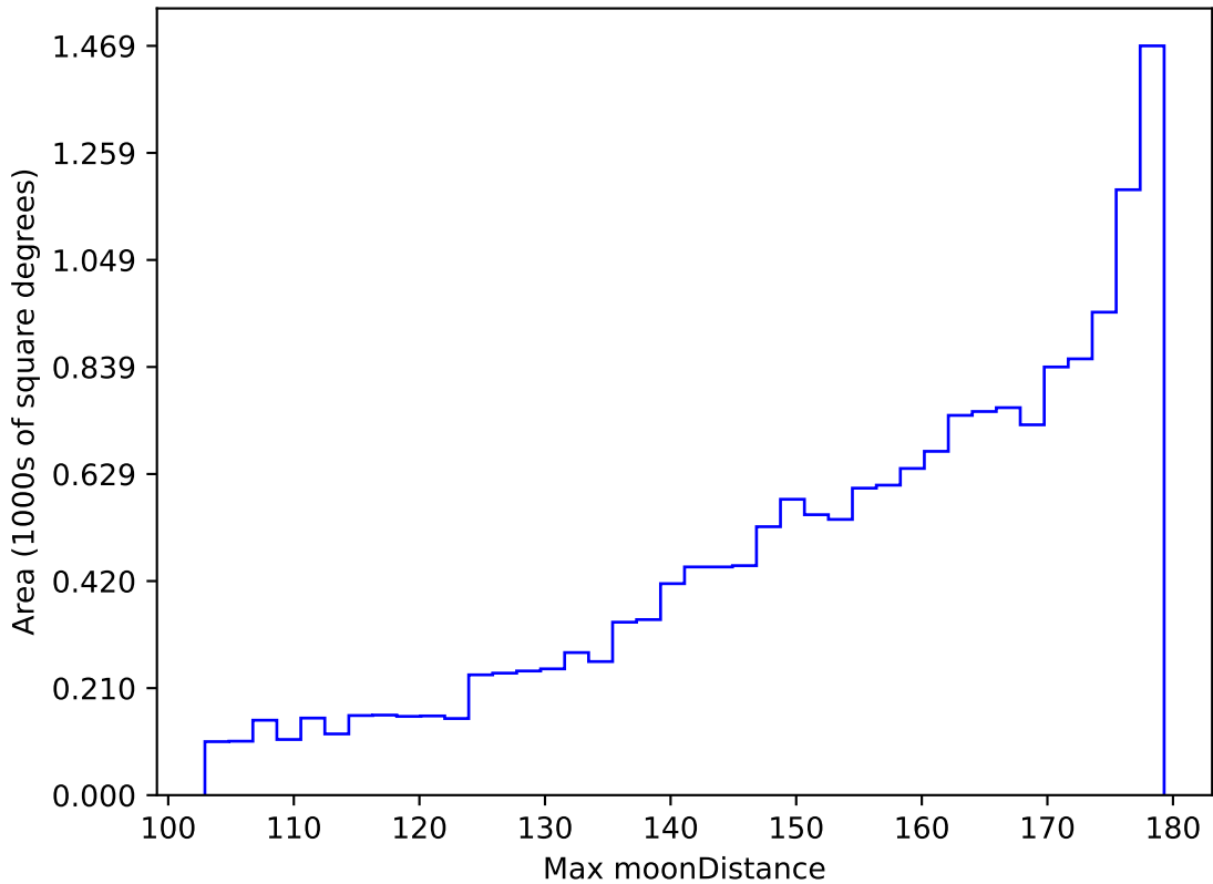
ddf_acor_sf30_lsf40_lsr20_v3.4_10yrs WFD i band: Max moonDistance
