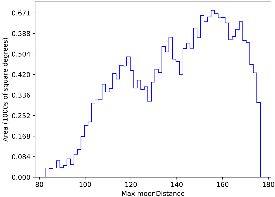
ddf_acor_sf30_lsf40_lsr20_v3.4_10yrs All sky y band: Max moonDistance
