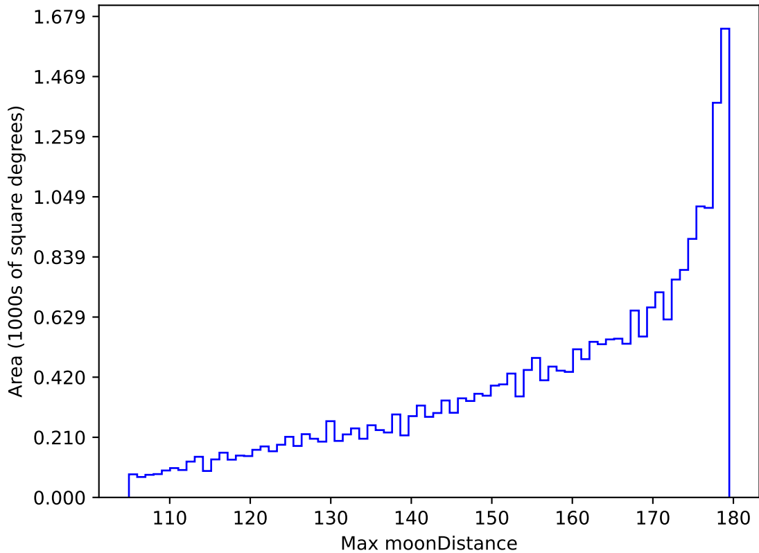
ddf_acor_sf30_lsf40_lsr20_v3.4_10yrs All sky all bands: Max moonDistance
