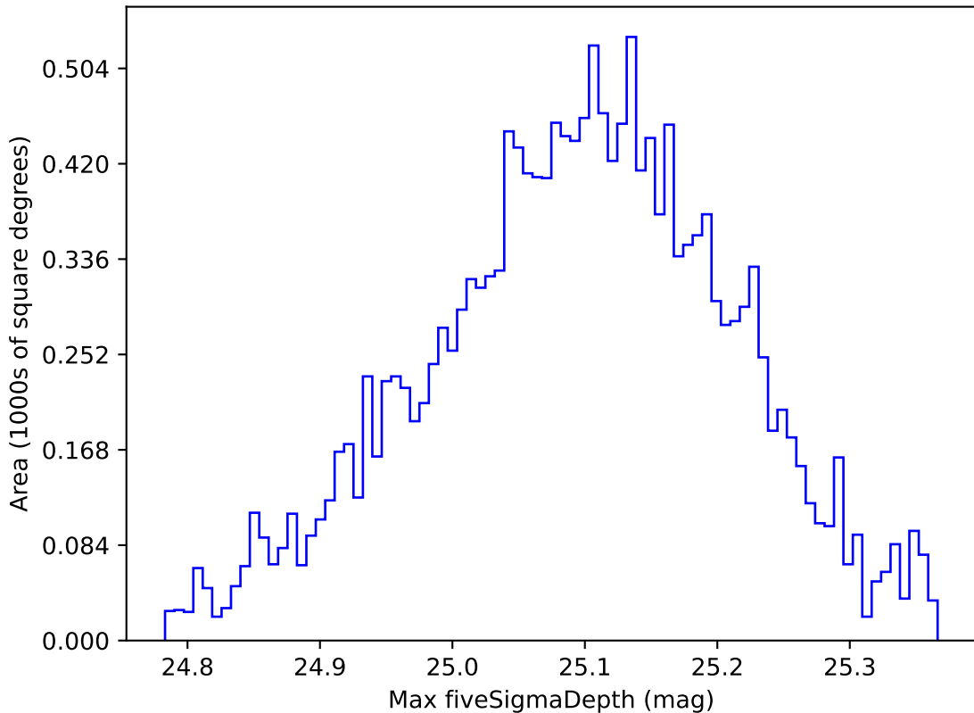
ddf_acor_sf30_lsf40_lsr20_v3.4_10yrs WFD all bands: Max fiveSigmaDepth
