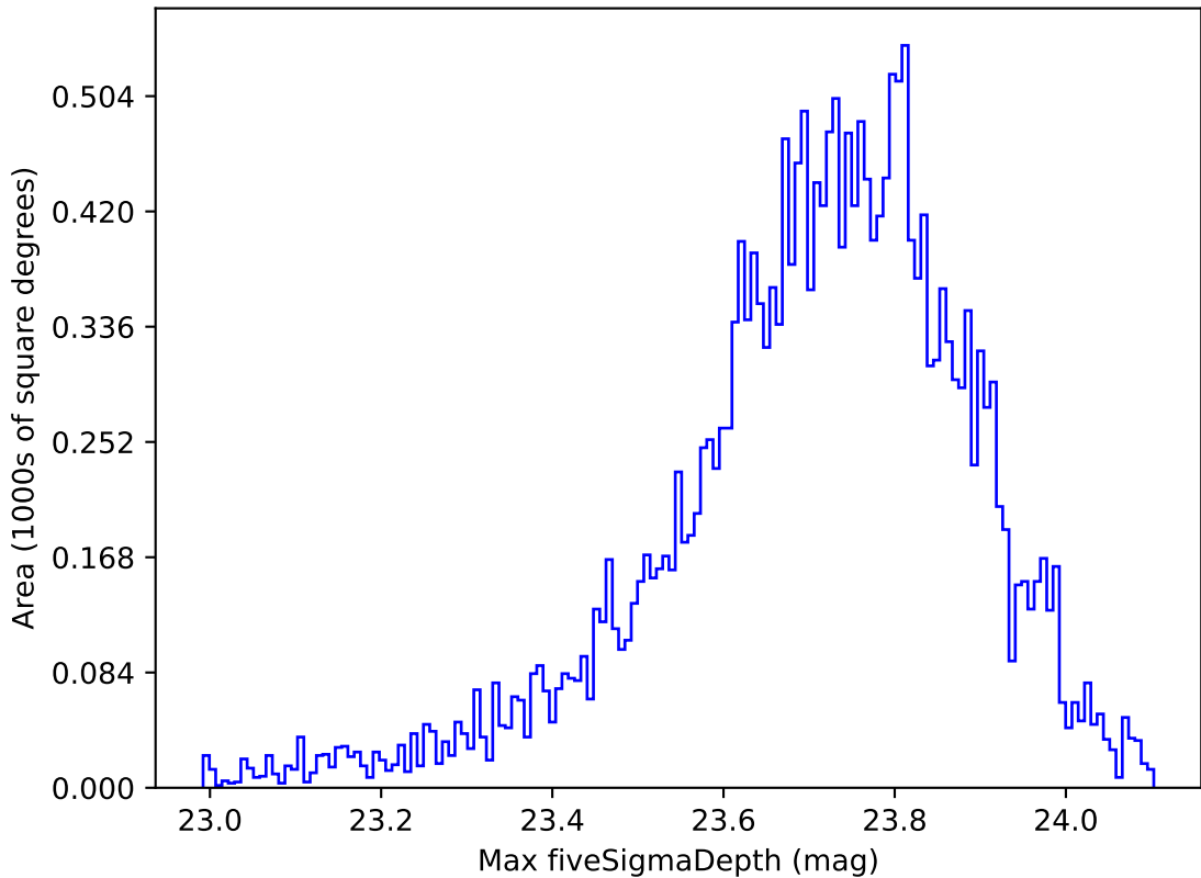
ddf_acor_sf30_ls40_lsr20_v3.4_10yrs All sky u band: Max fiveSigmaDepth
