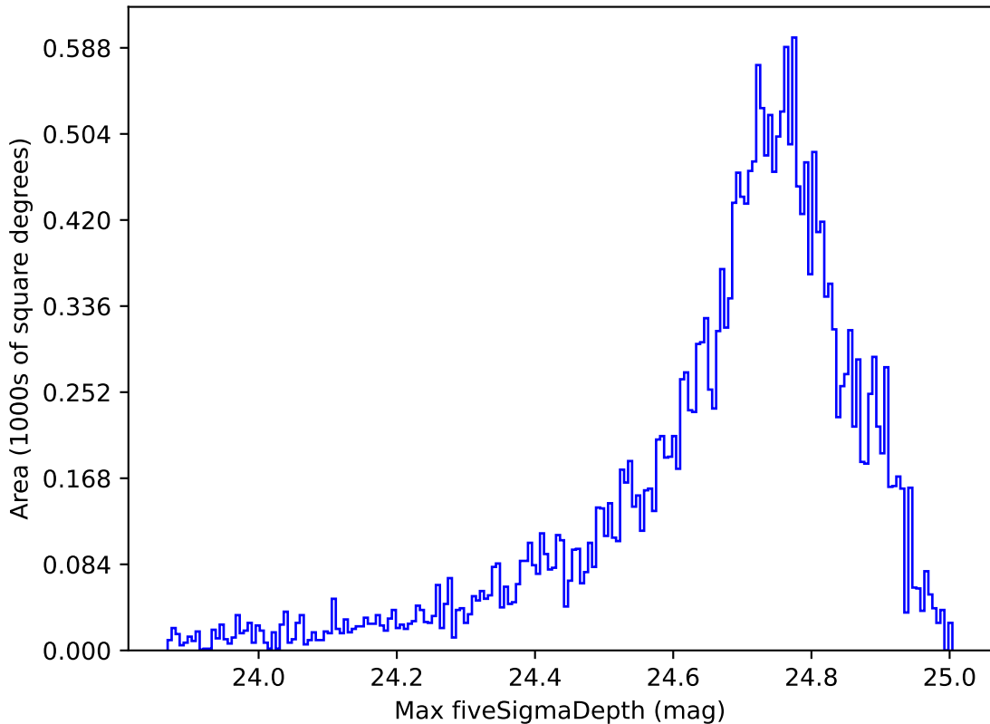
ddf_acor_sf30_lsf40_lsr20_v3.4_10yrs All sky r band: Max fiveSigmaDepth
