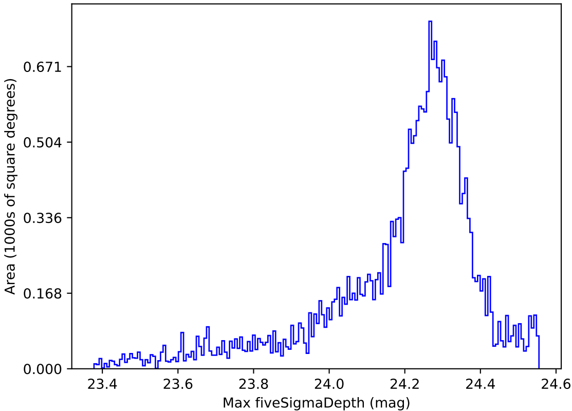
ddf_acor_sf30_lsf40_lsr20_v3.4_10yrs All sky i band: Max fiveSigmaDepth
