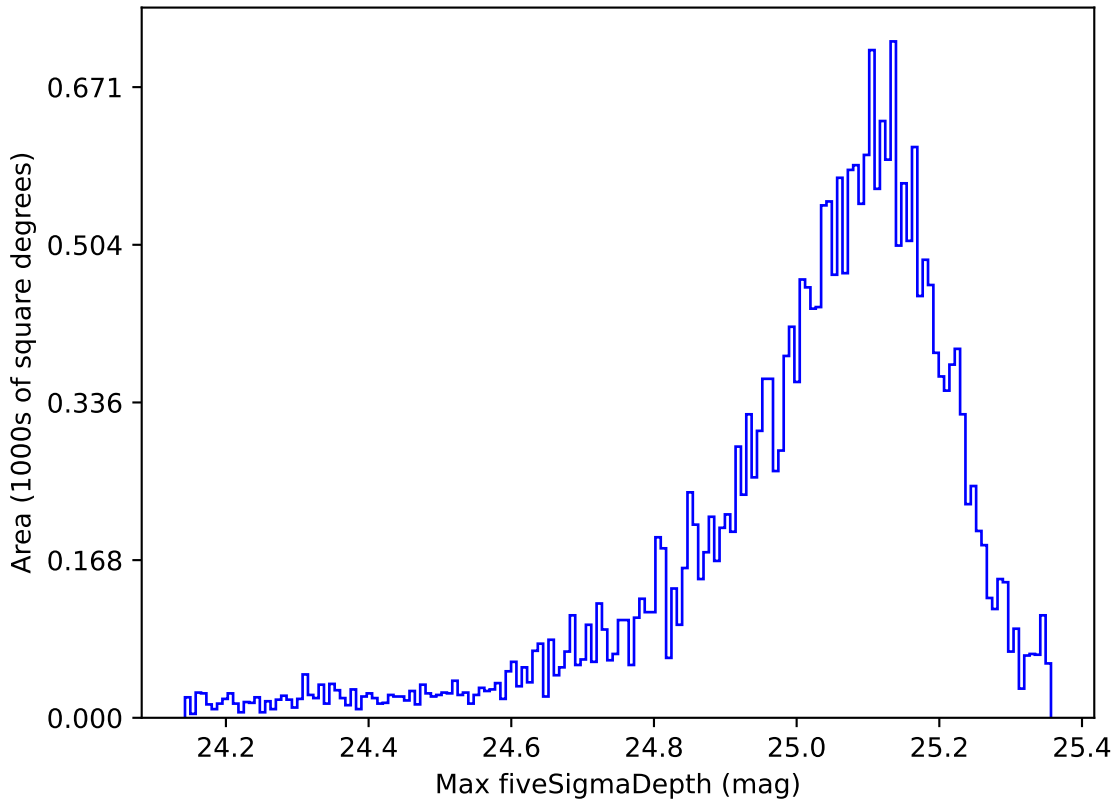
ddf_acor_sf30_lsf40_lsr20_v3.4_10yrs All sky g band: Max fiveSigmaDepth
