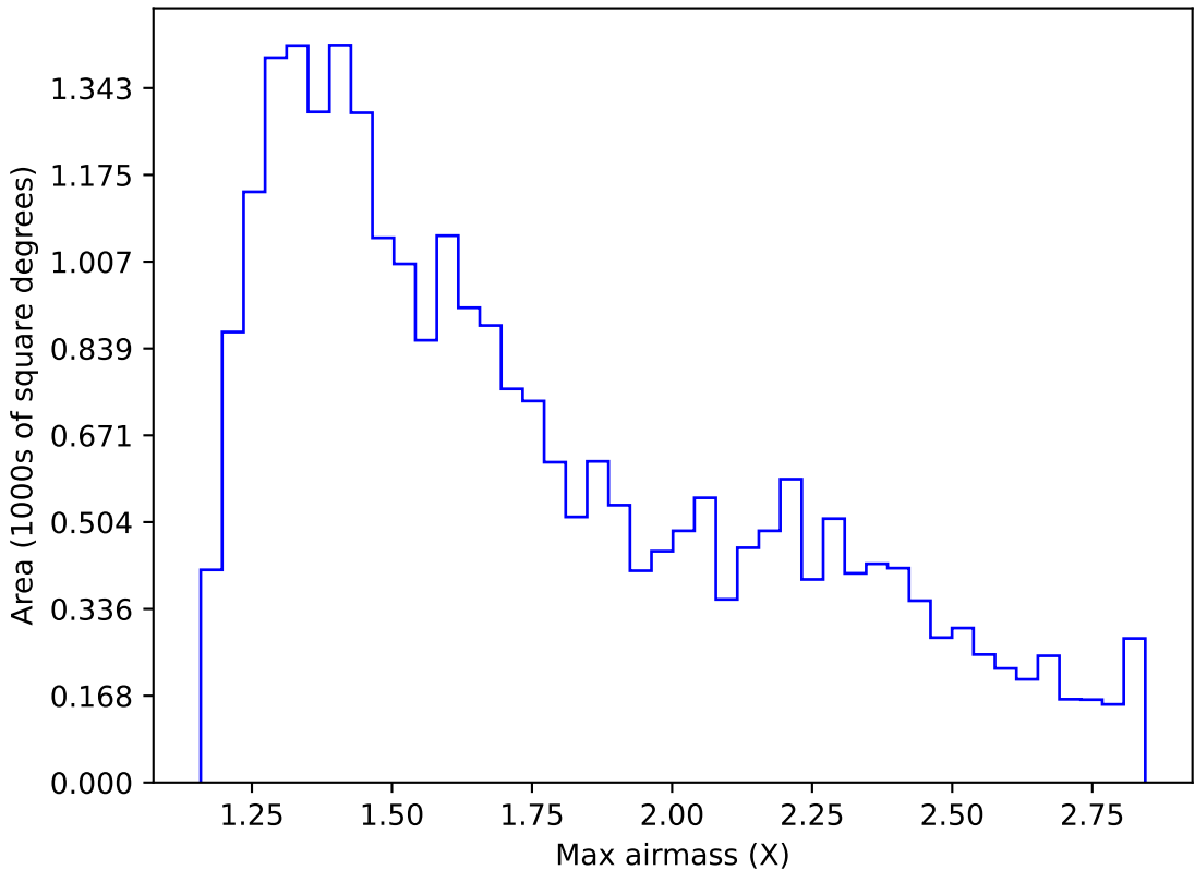
ddf_acor_sf30_lsf40_lsr20_v3.4_10yrs Yr 1 z band: Max airmass
