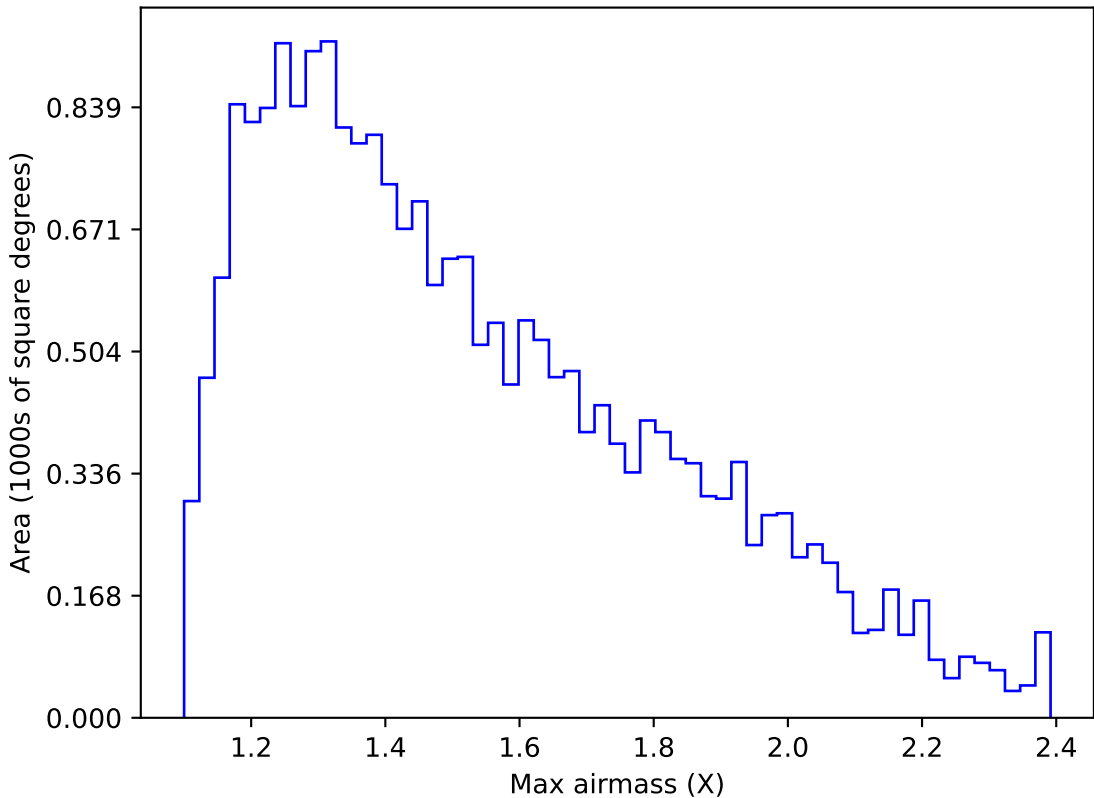
ddf_acor_sf30_lsf40_lsr20_v3.4_10yrs Yr 1 u band: Max airmass
