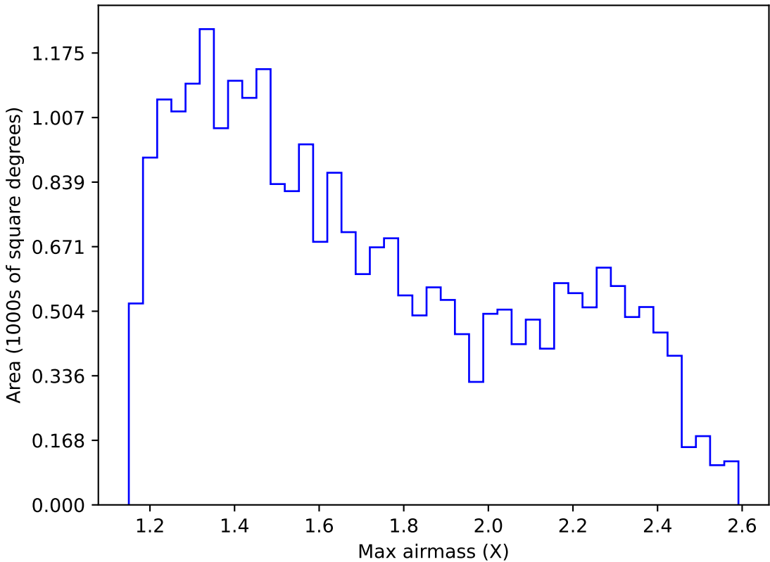
ddf_acor_sf30_lsf40_lsr20_v3.4_10yrs Yr 1 r band: Max airmass
