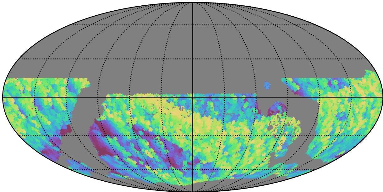
ddf_acor_sf30_lsf40_lsr20_v3.4_10yrs WFD z band: Max airmass
