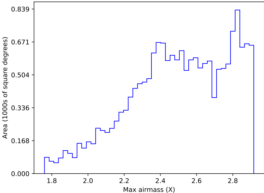
ddf_acor_sf30_lsf40_lsr20_v3.4_10yrs WFD z band: Max airmass
