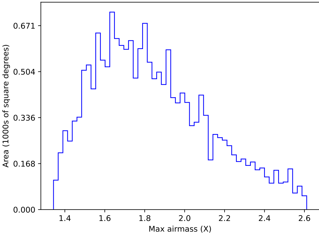
ddf_acor_sf30_lsf40_lsr20_v3.4_10yrs WFD u band: Max airmass
